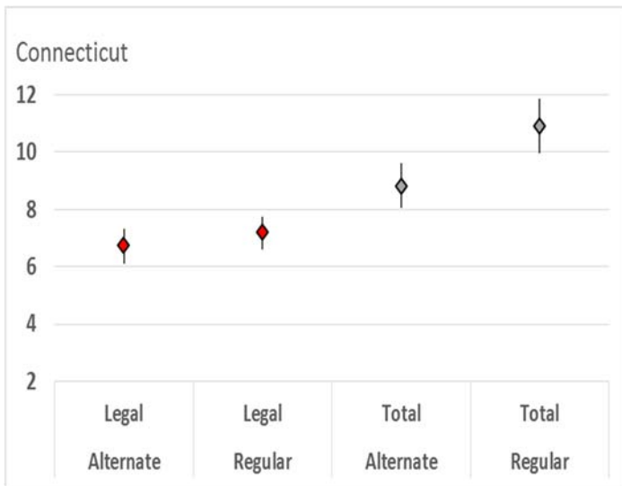
Figure 1(A): ANOVA results of bait trials in Connecticut. Graphs show mean conch catch per trap (diamond) and 95% confidence intervals (bars).
