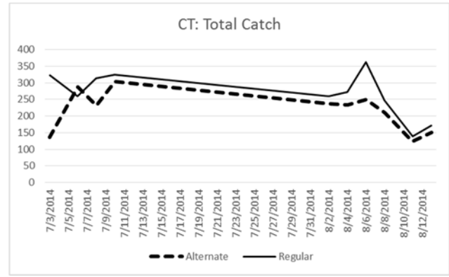
Figure 2: Total conch catch in numbers for equal numbers of traps using each bait type by date for trials in Rhode Island and Connecticut.
