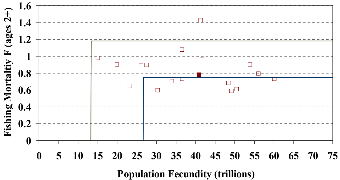
Figure 8. Control plot of F and SSB from base Beverton-Holt run in current assessment for Atlantic menhaden with newly recommended benchmarks (solid square represents 2002) (2003 Stock Assessment).
