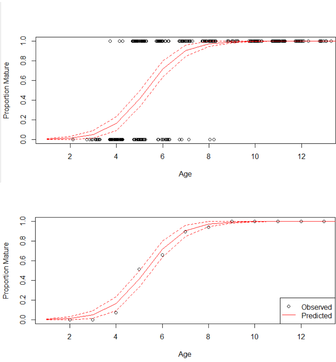
Figure B5.1. Estimated proportions mature, by age, for the March-July dataset. Developing fish are considered not imminently spawning. Top figure shows the sample size and maturity status for each fish sampled, by age, and bottom figure shows the overall observed proportion mature.
