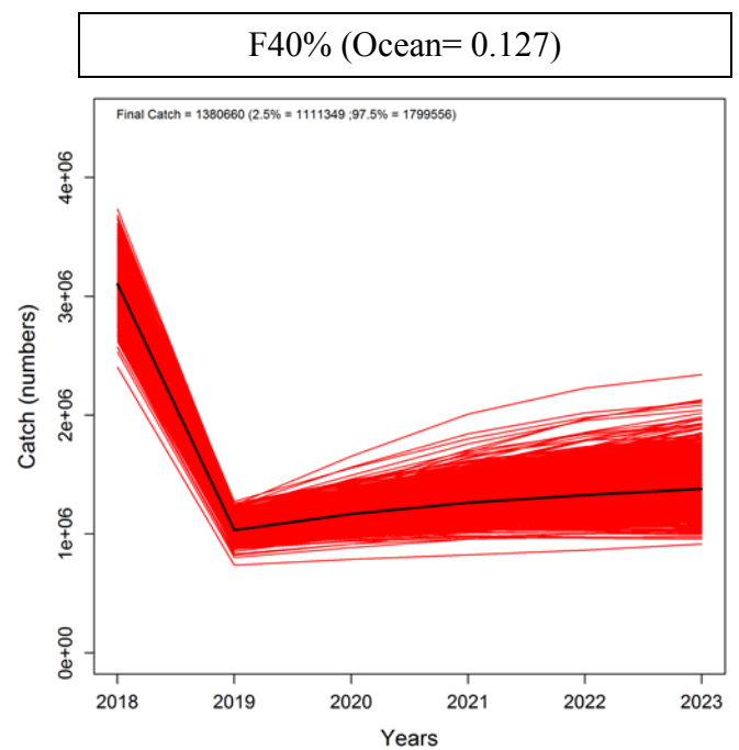
Figure B10.5. Projected total catch from the Delaware Bay/Hudson River stock under different fishing mortality scenarios using the hockey-stick female spawning stock biomass-recruitment approach. F_{2018} was assumed equal to F_{2017} in all scenarios.
