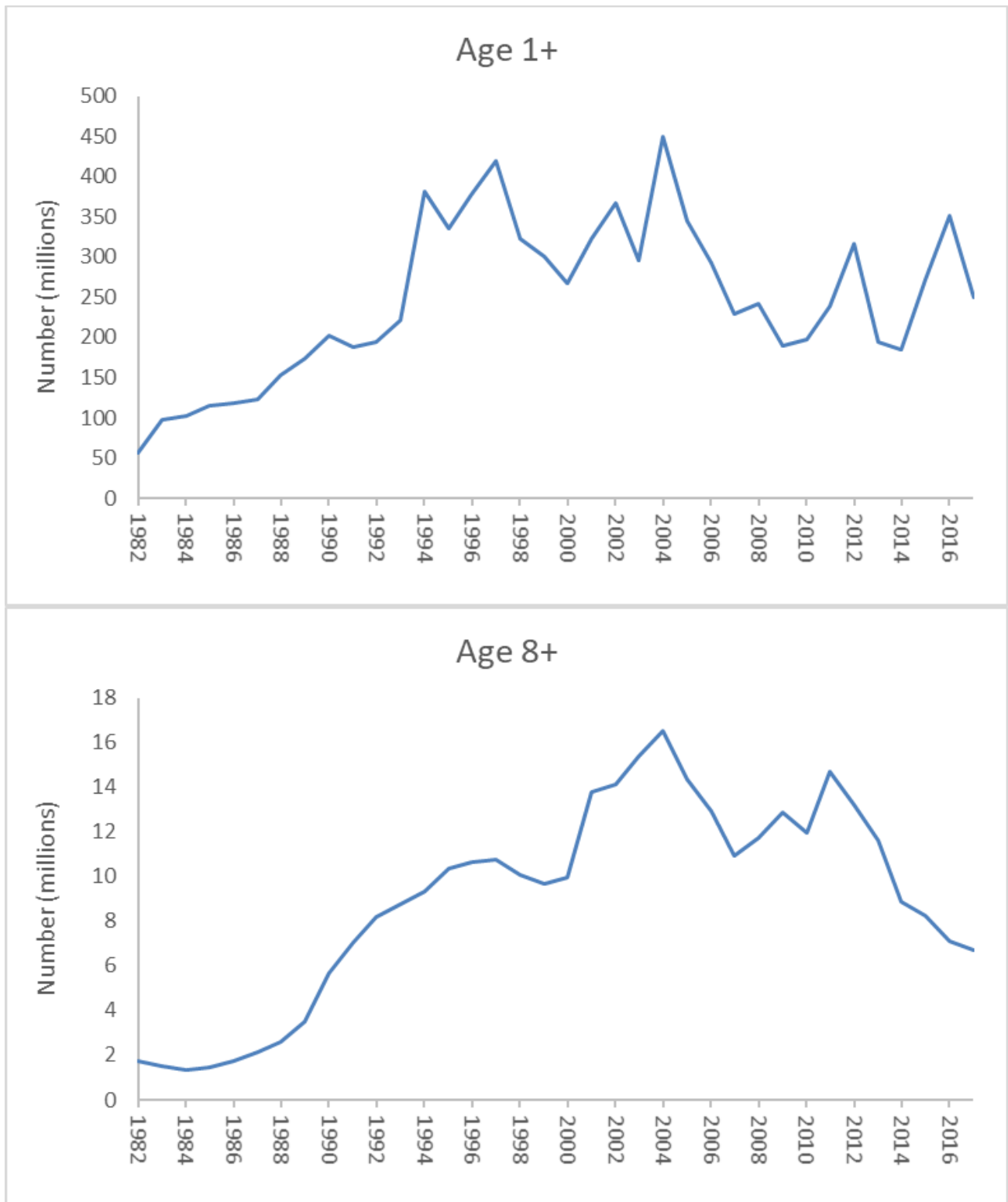
Figure B7.30. Estimates of January-1 total (age 1+) and 8+ abundance for 1982-2017 from the non-migration SCA.
