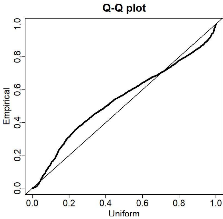
Figure 7. Q-Q-plot for ASMFC Summer Survey residuals.
