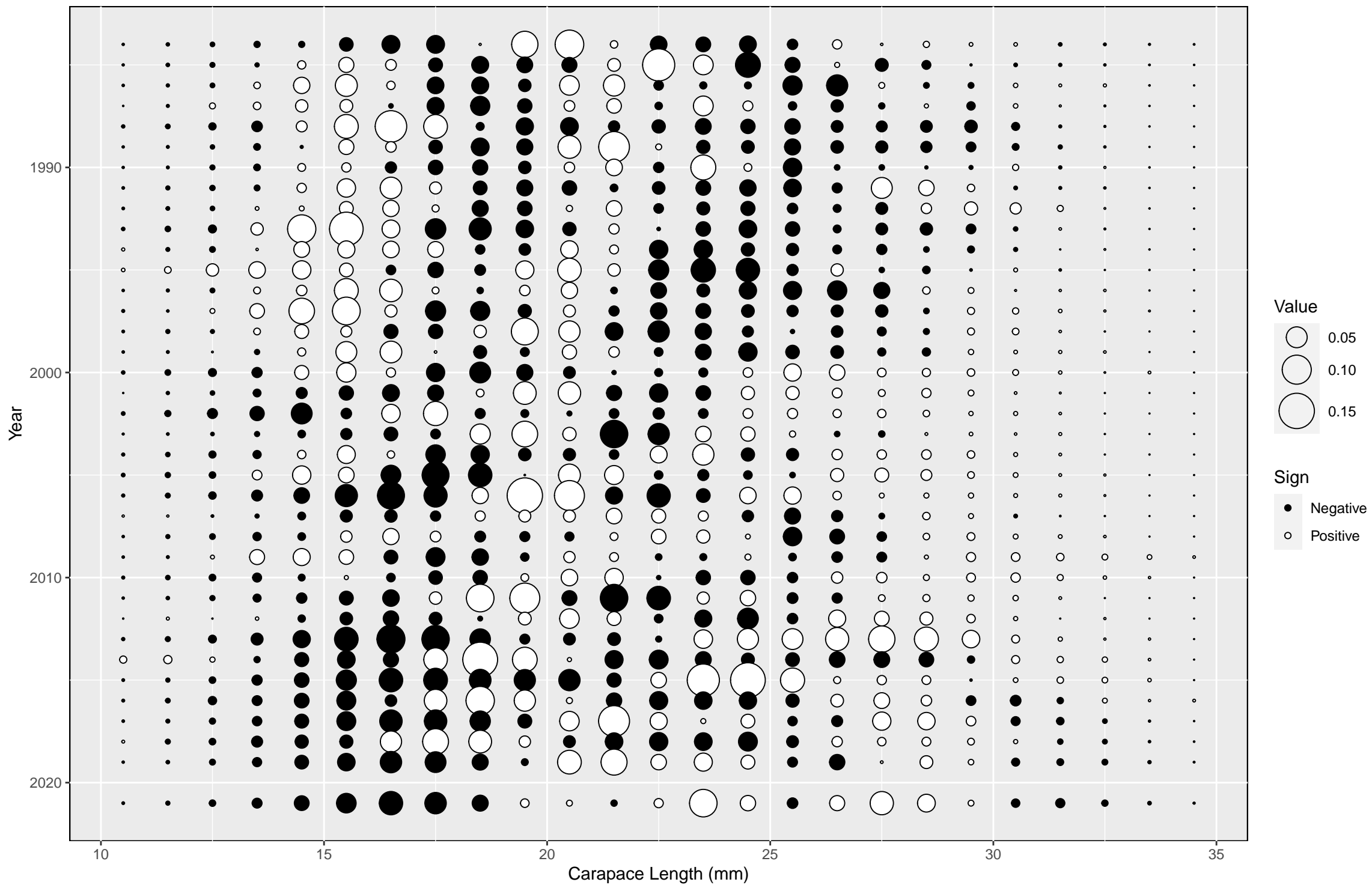
Length Composition Residuals – ASMFC Shrimp Survey
