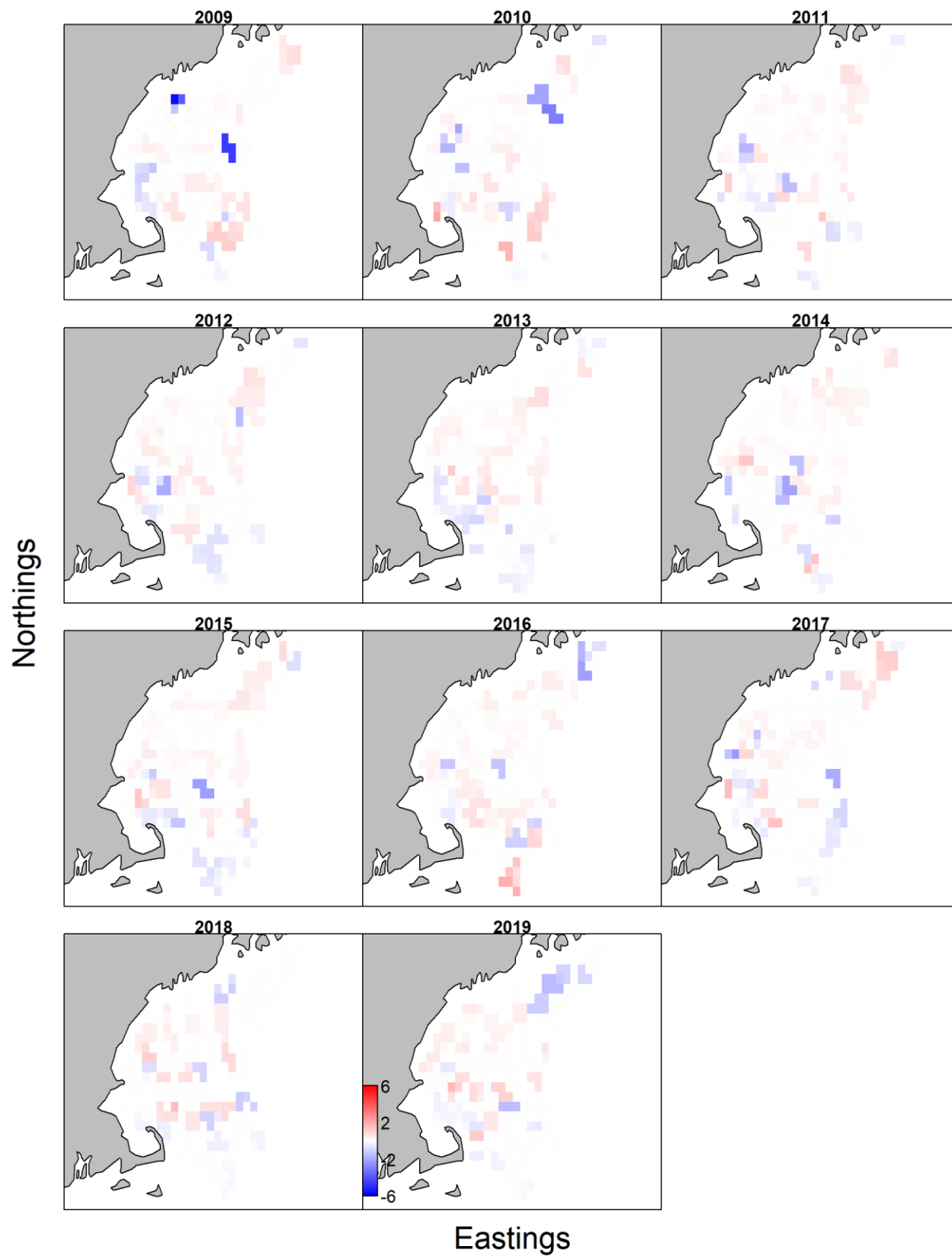
Figure 13. Annual total catch Pearson residuals by area for the NEFSC Fall Survey.
