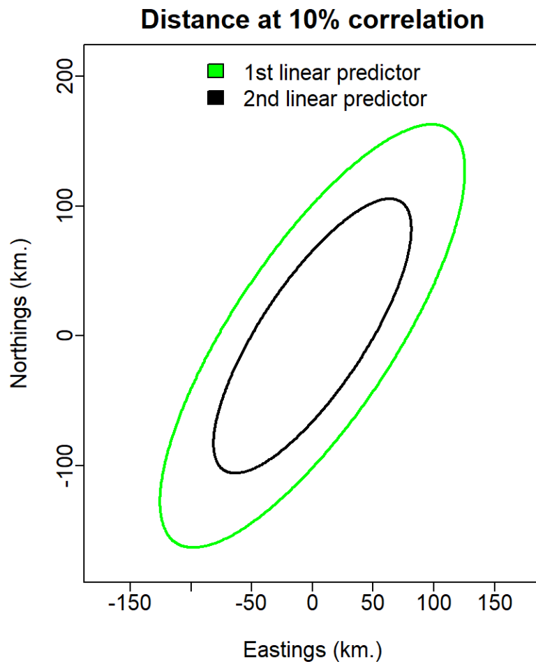
Figure 16. Direction of geometric anisotropy for the NEFSC Fall Survey.
