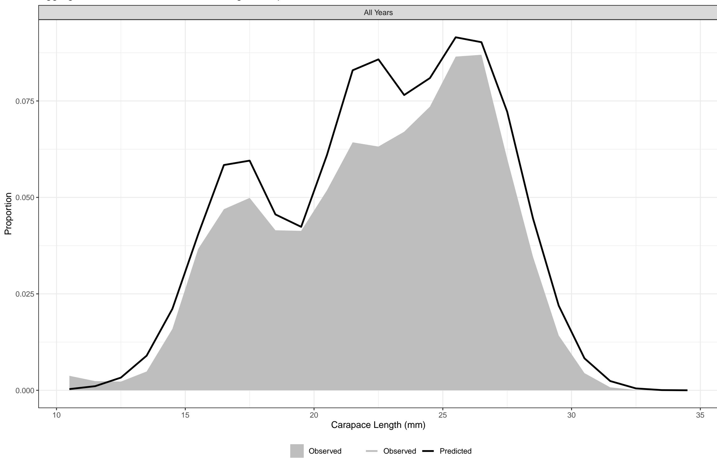
Aggregated Observed and Predicted Length Composition – NEFSC Fall Trawl
