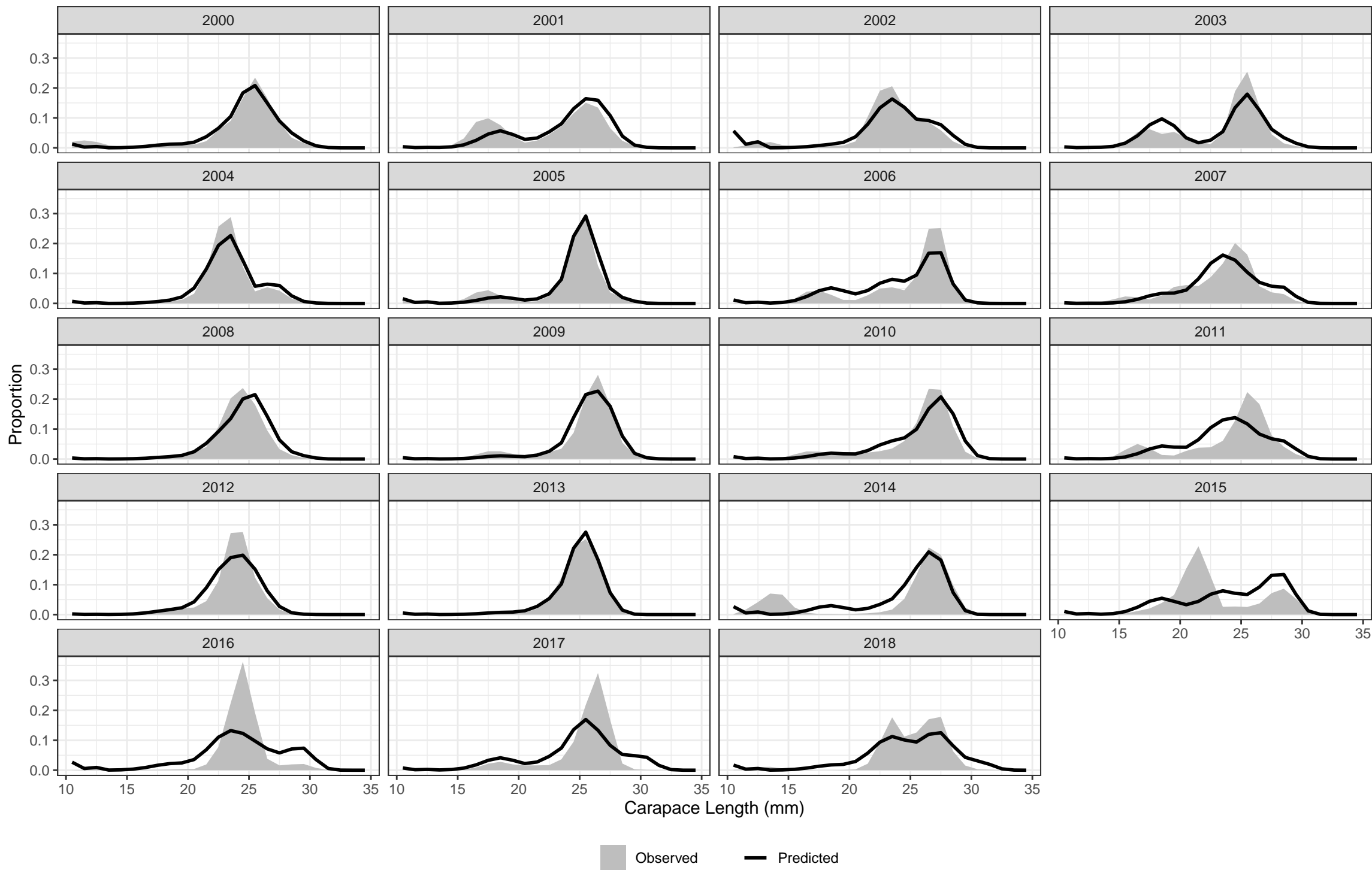
Observed and Predicted Length Composition – Trawl Fleet
