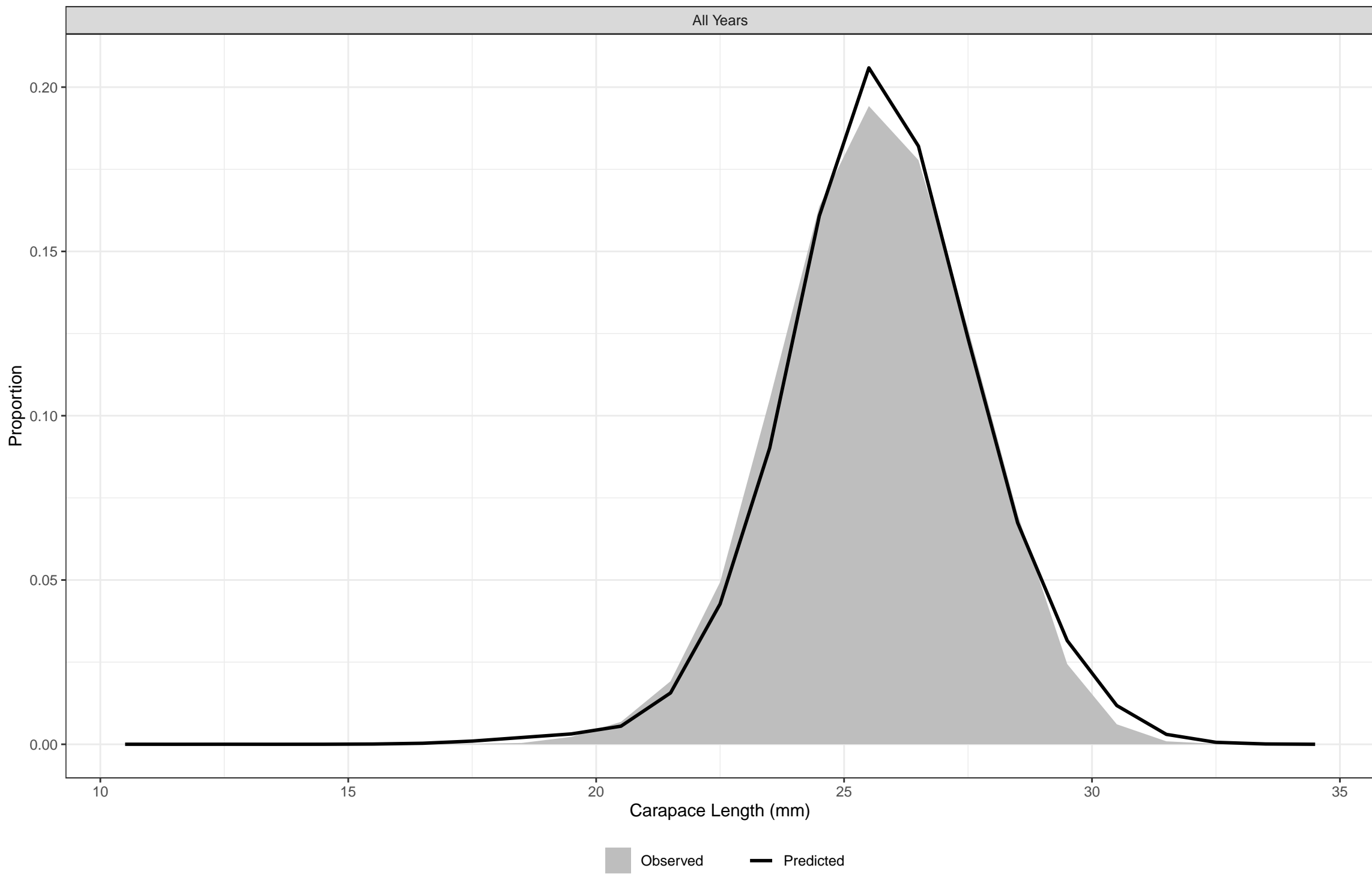
Aggregated Observed and Predicted Length Composition – Trap Fleet
