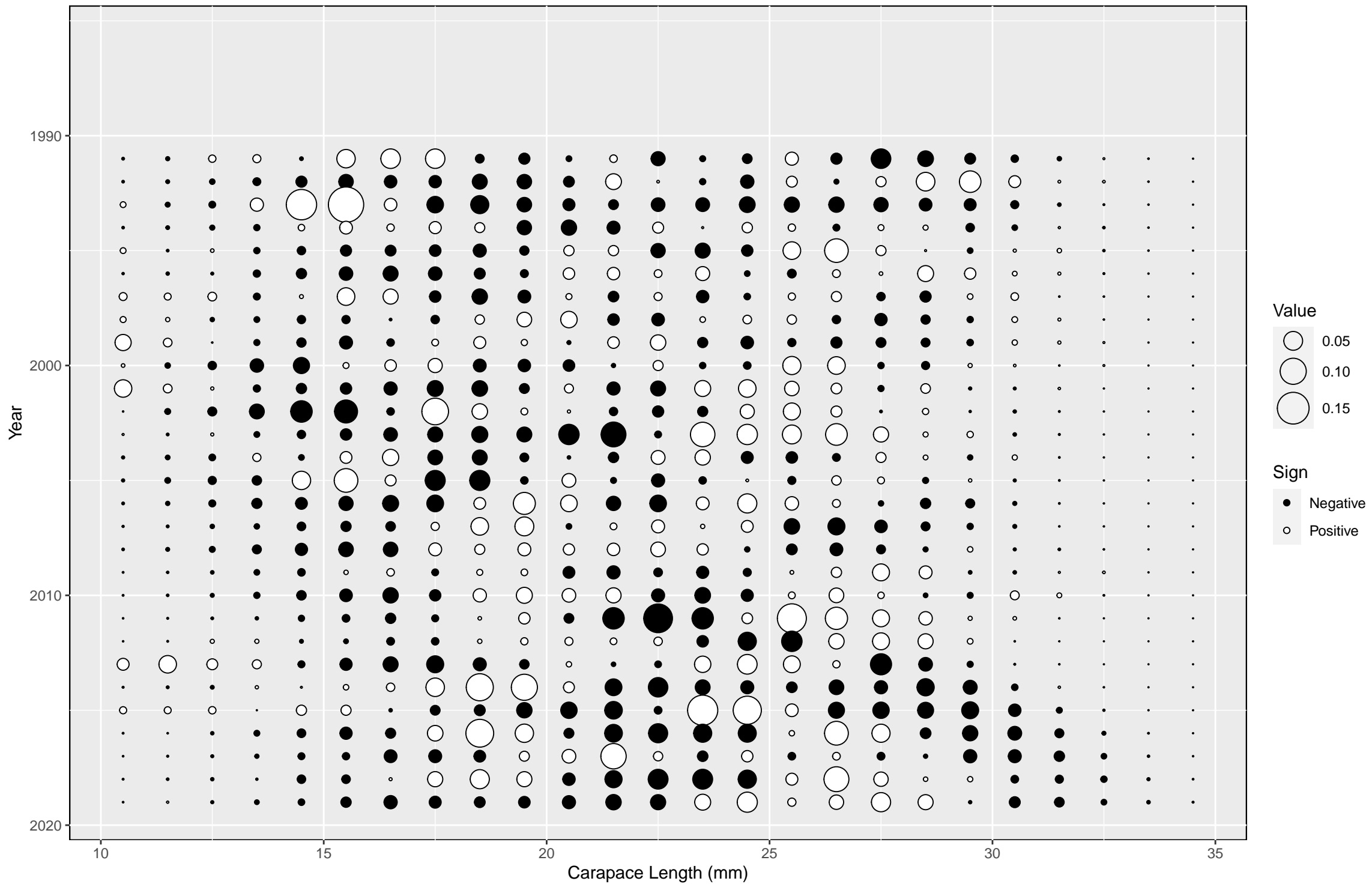
Length Composition Residuals – NEFSC Fall Trawl
