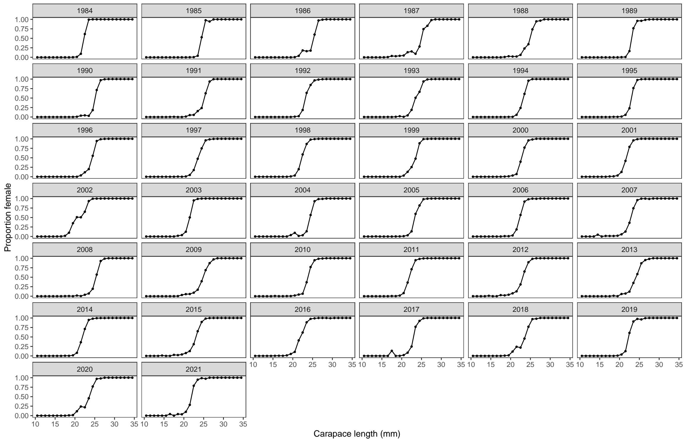
Proportion Female at Length
