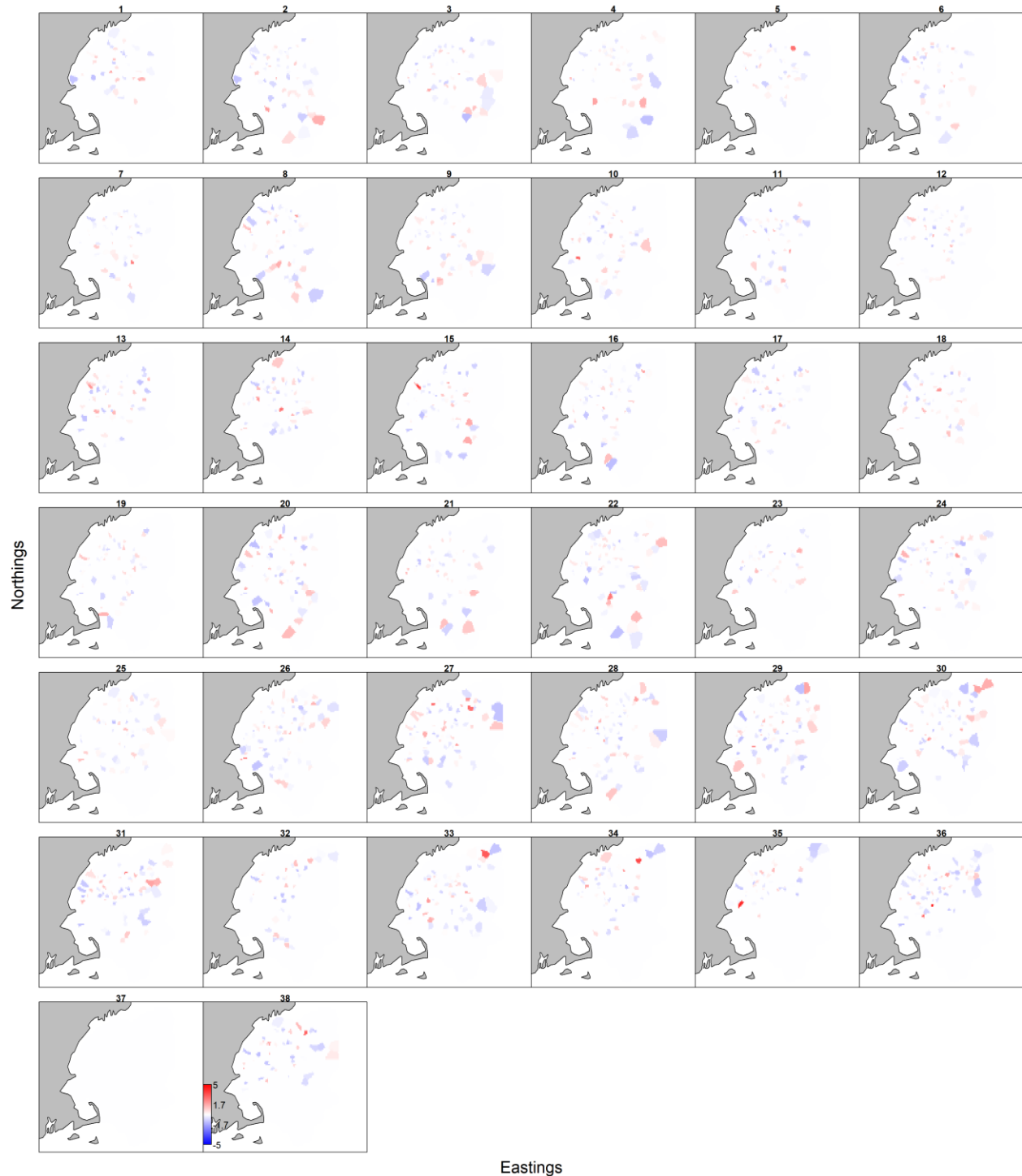
Figure 5. Annual total catch Pearson's residuals by area for the ASMFC Summer Survey.
