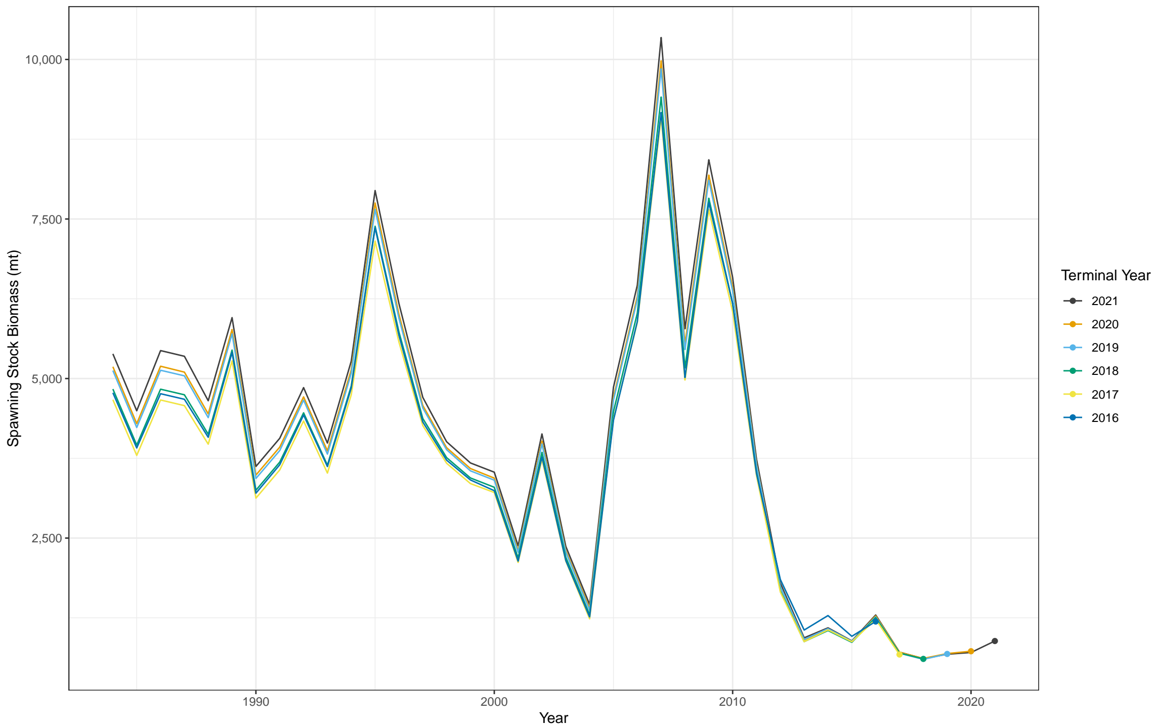
Spawning stock biomass retrospective – absolute
