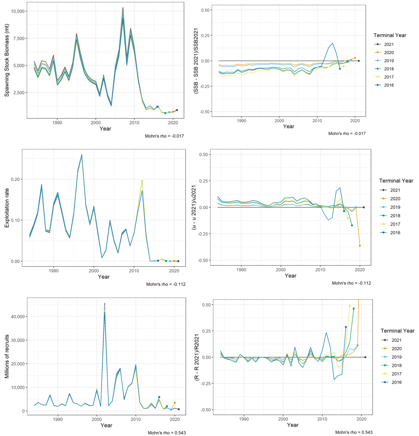
Figure 13. Retrospective analysis of UME model results for spawning stock biomass (top), exploitation rate (middle), and recruitment (bottom).
