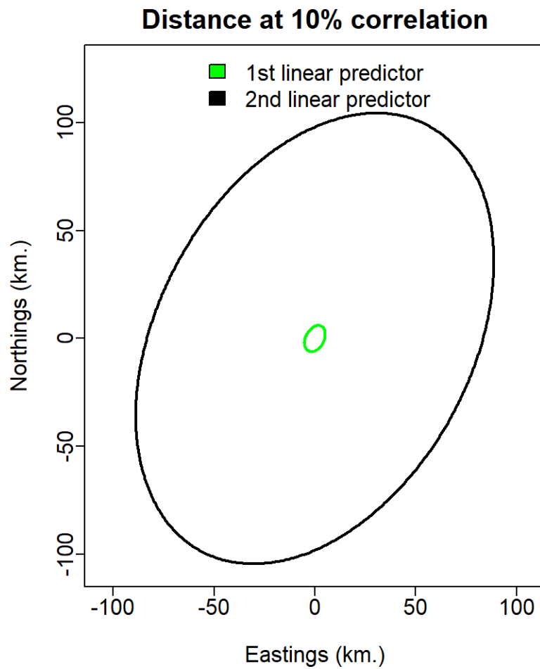
Figure 8. Direction of geometric anisotropy for the ASMFC Summer Survey.
