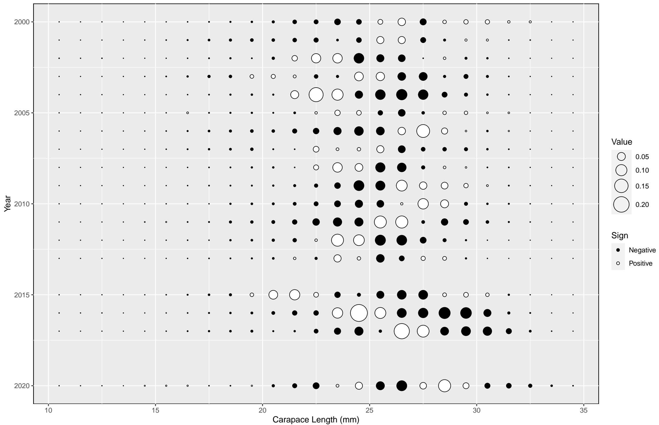
Length Composition Residuals – Trap Fleet
