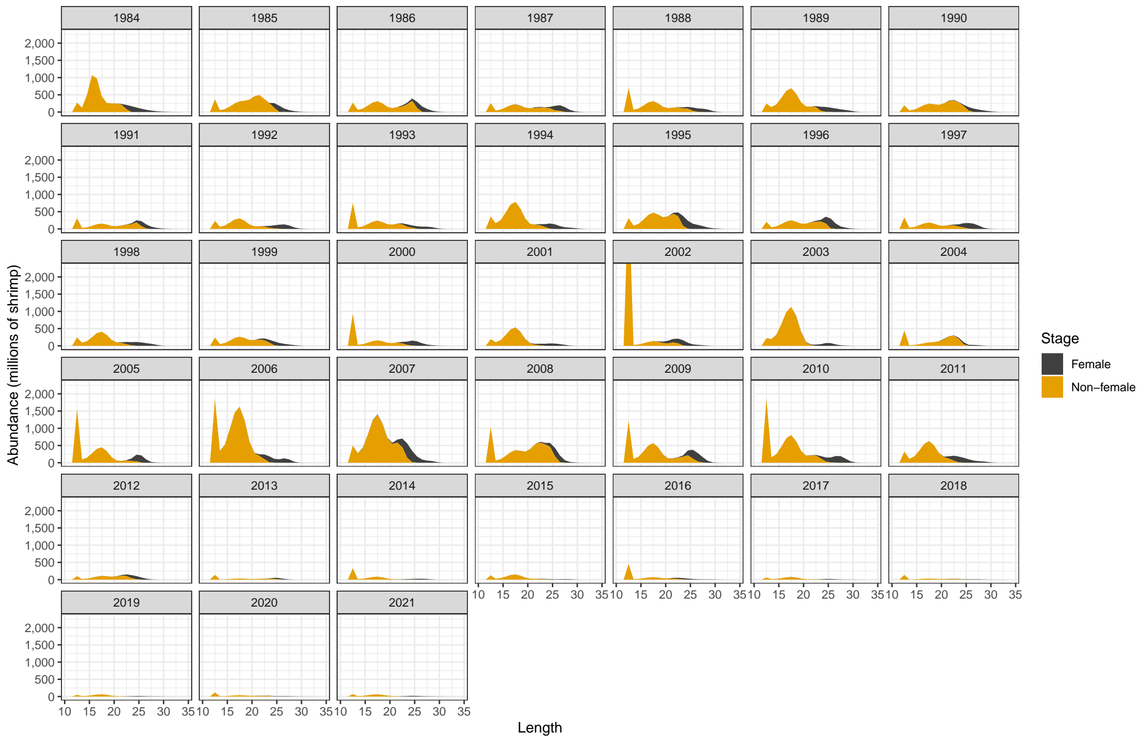
Abundance at Length by Stage
