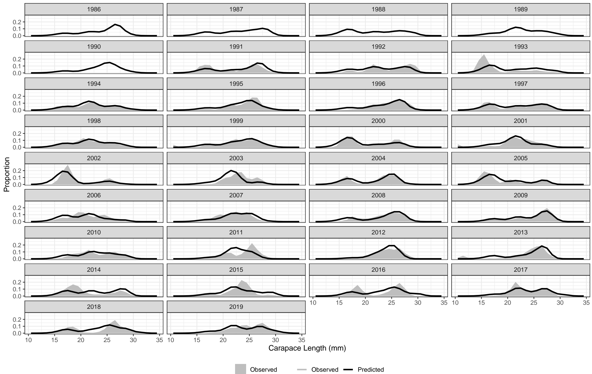
Observed and Predicted Length Composition – NEFSC Fall Trawl
