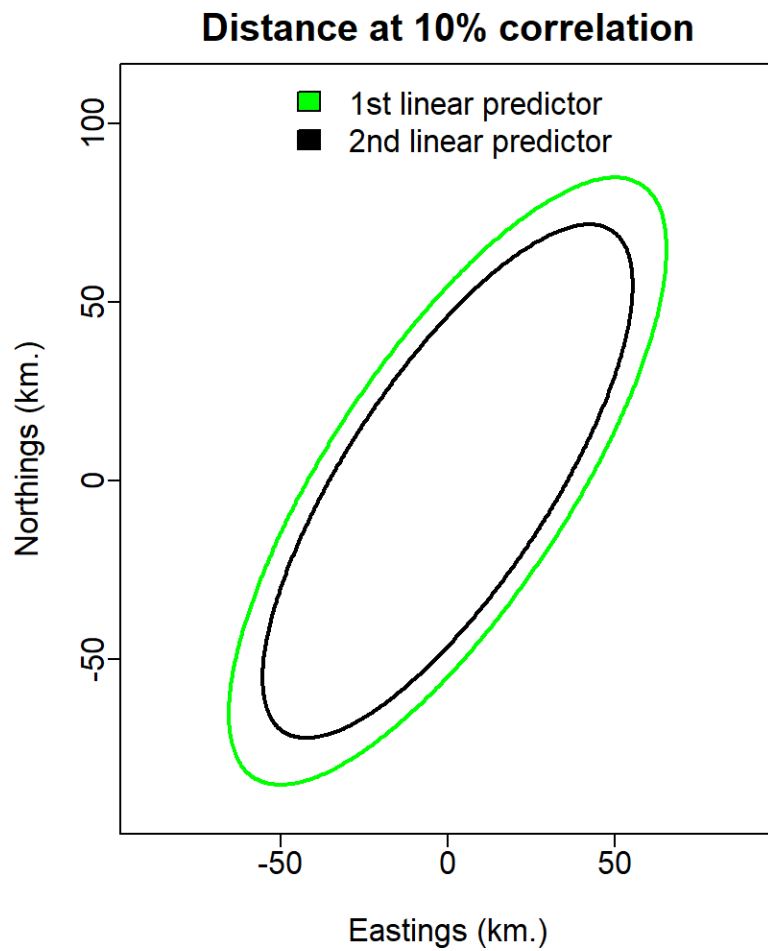
Figure 24. Direction of geometric anisotropy for the ME-NH Spring Survey.
