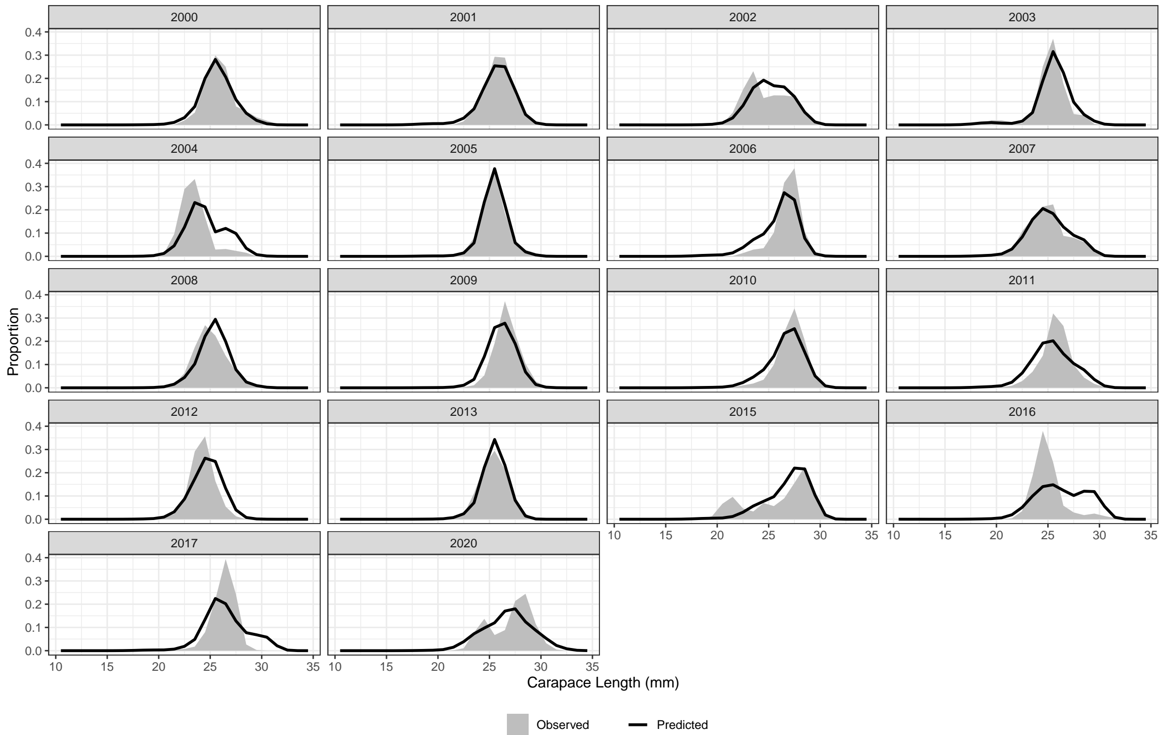
Observed and Predicted Length Composition – Trap Fleet
