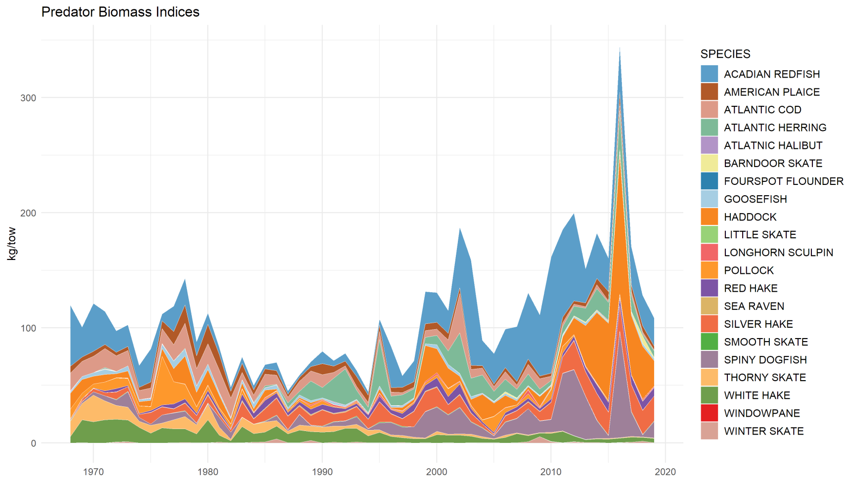
Figure 4. Biomass indices of the key northern shrimp predators used to develop the predation pressure index (PPI) used in the assessment.
