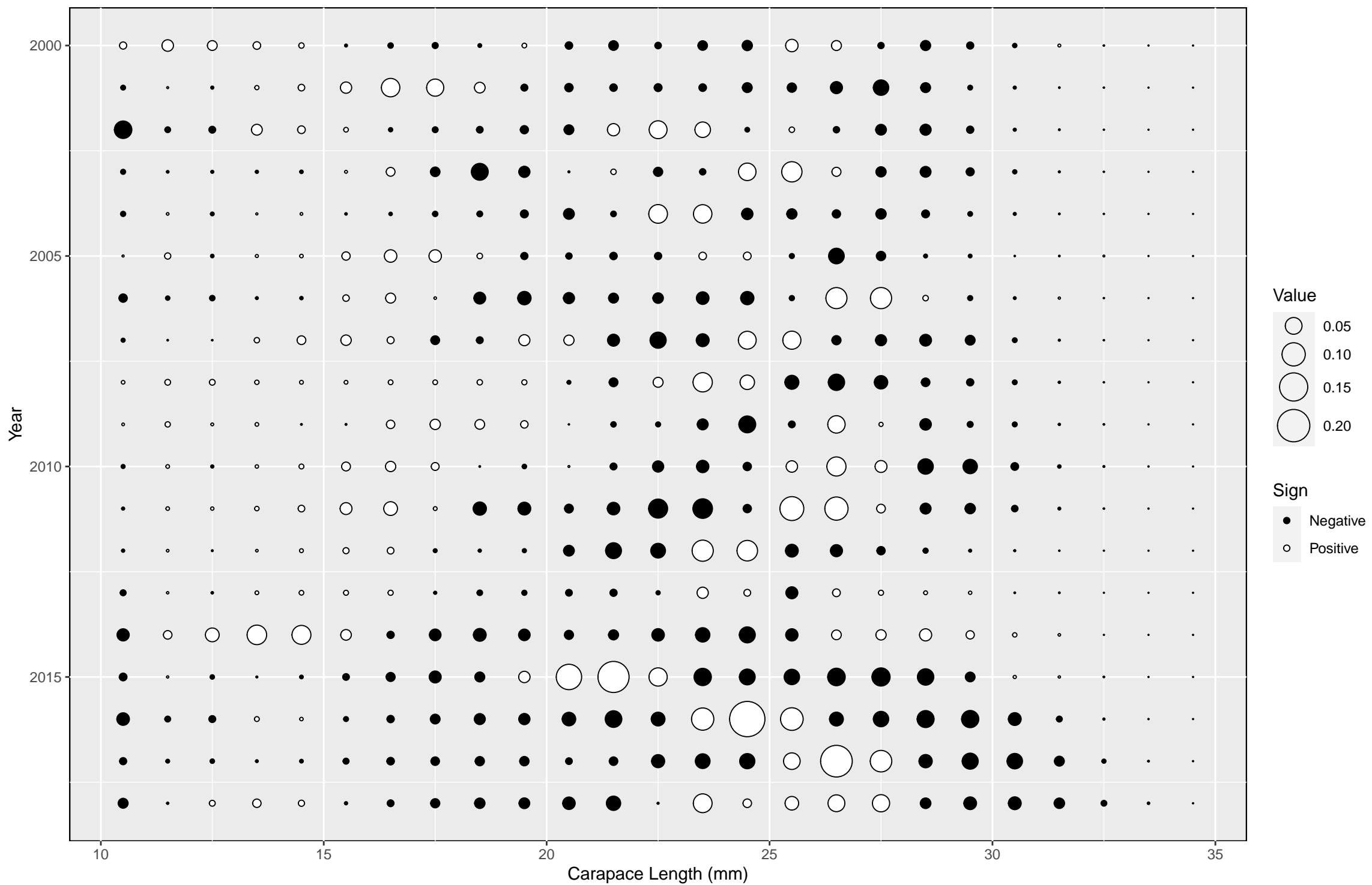
Length Composition Residuals – Trawl Fleet
